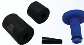
3871 Ford Fuel injector Seal Installer
