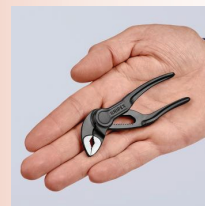
87 00 100 Cobra XS • Only 4" in length • 1" gripping capacity • 11 adjustment positions
